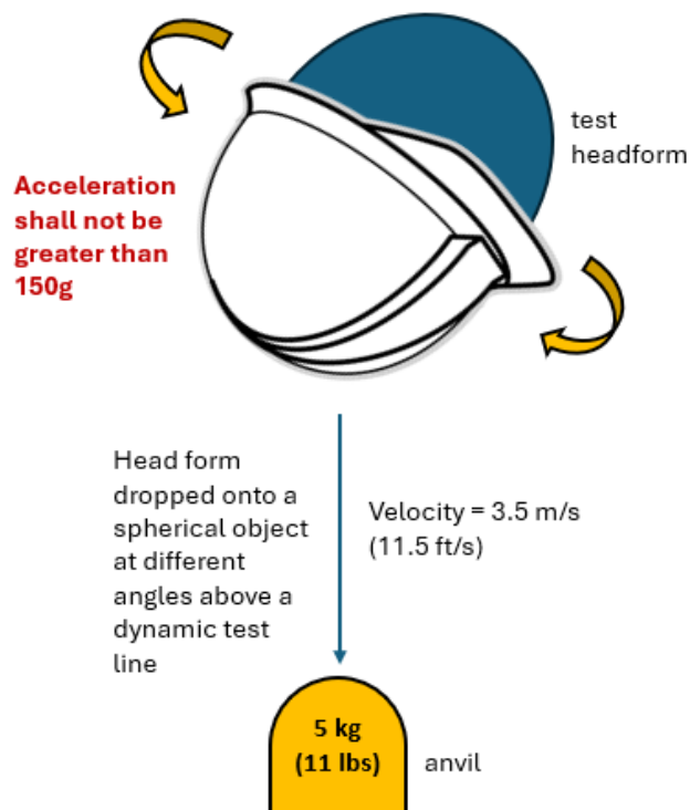
Figure 3: TYPE II ONLY IMPACT ENERGY ATTENUATION
