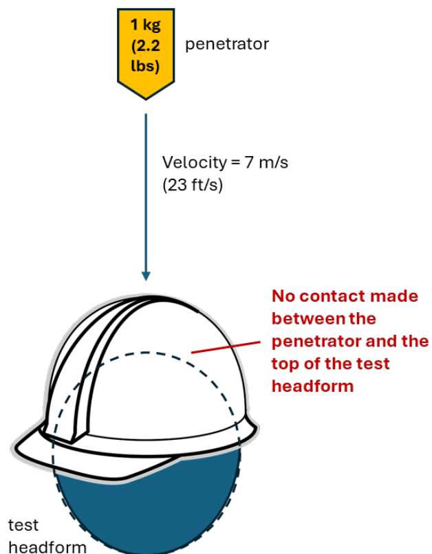
Figure 2: TYPE I & TYPE II APEX PENETRATION TESTING
